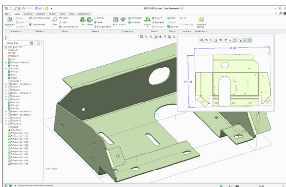
Flat pattern previews in sheetmetal design in Creo Parametric update dynamically so you can see your design edits in real-time.
